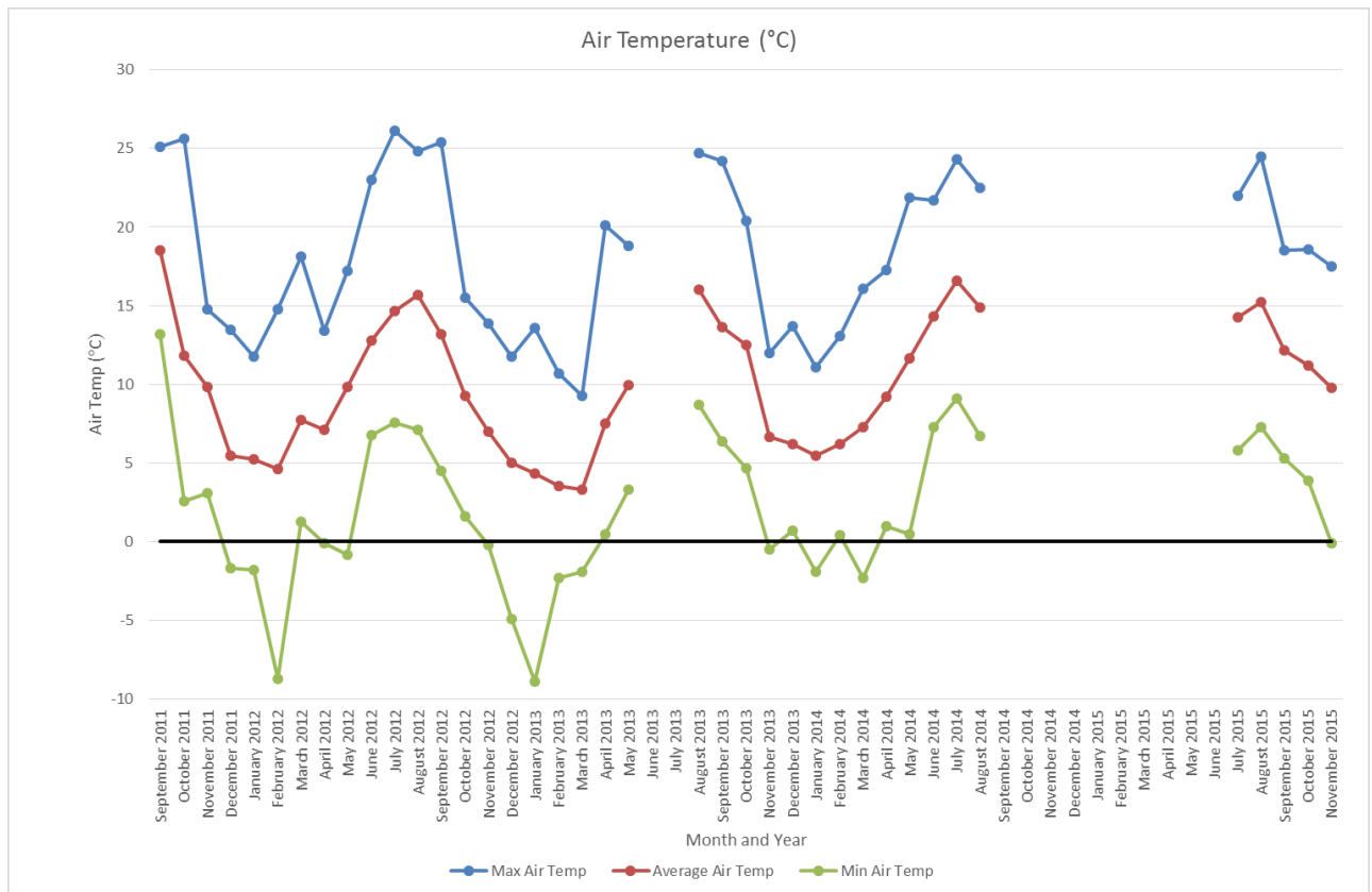
Figure 2.6 Air temperature variation (2011 to 2015)
