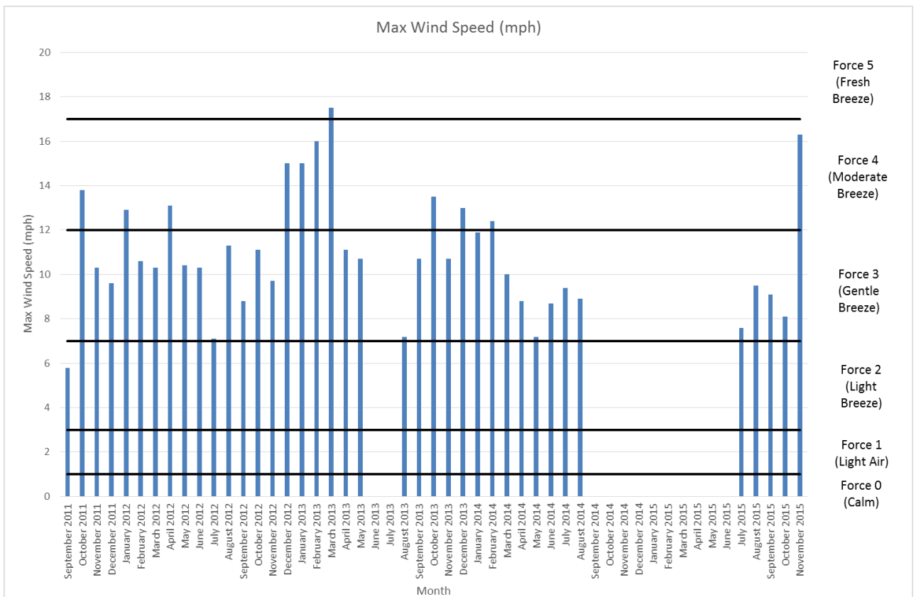
Figure 2.5 Maximum daily wind speed (2011 to 2015)
