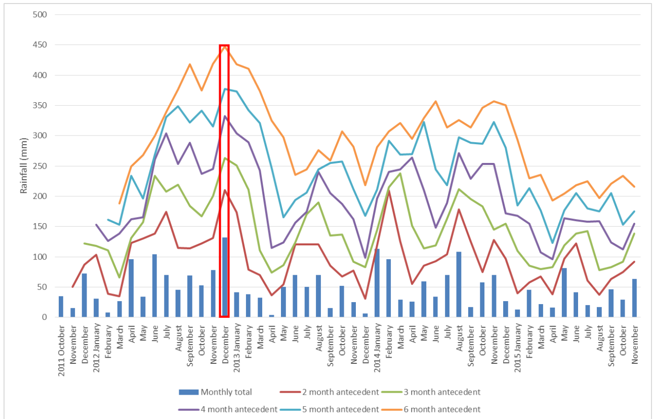
Figure 2.7. Monthly rainfall and antecedent totals (2011 to 2015). Ground movements were recorded at Scalby Mills during December 2012 (red box).
