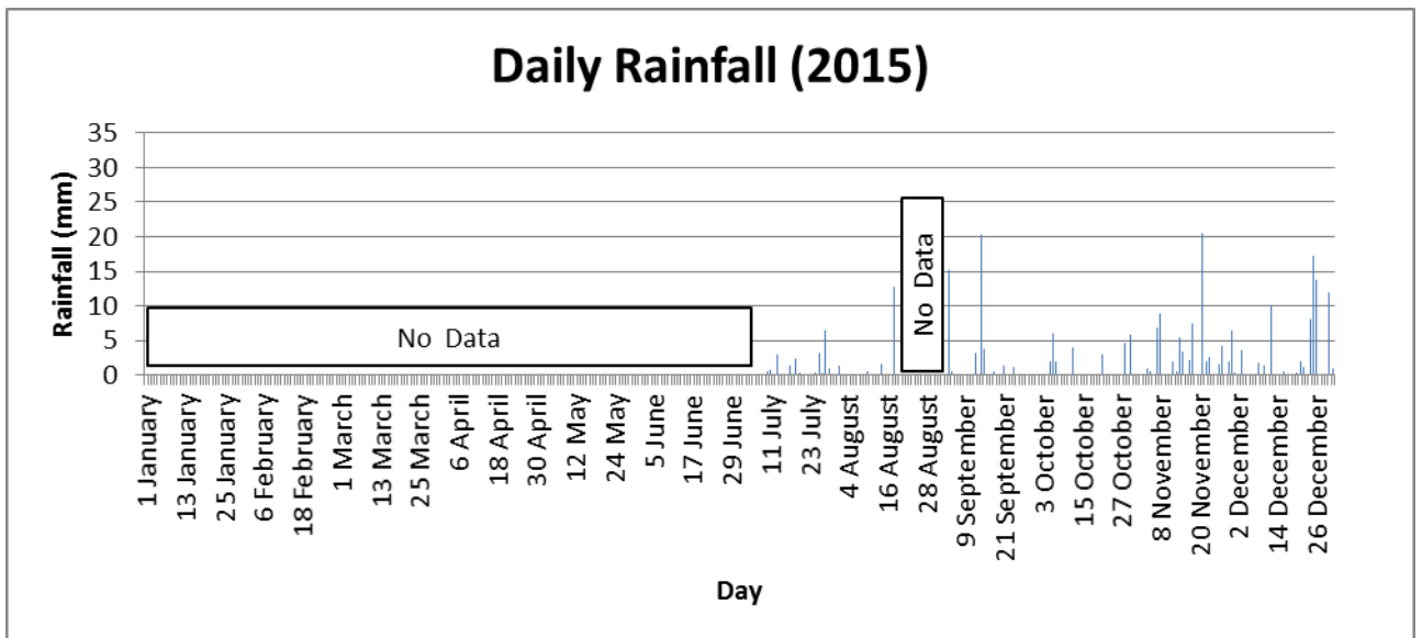
Figure 2.3 Daily rainfall recorded at Flat Cliffs during 2015
