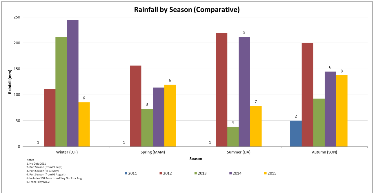
Figure 2.4 Seasonal rainfall comparison (2011-2015)
