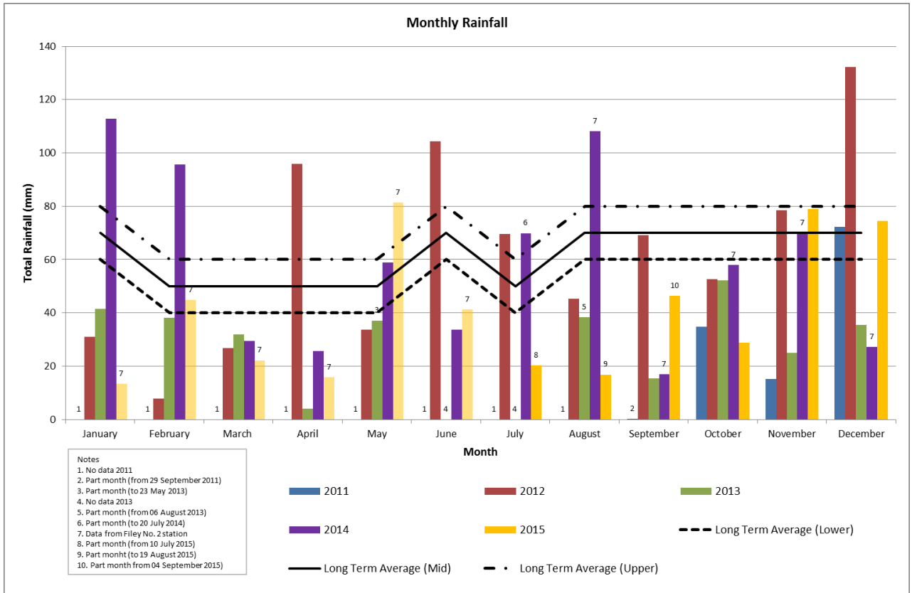
Figure 2.2 Comparison of monthly rainfall records (2011 to 2015).
