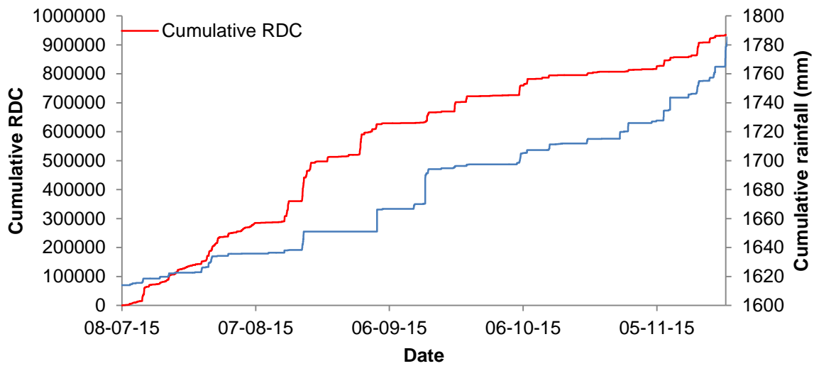
Figure 9.2. AE rate- and cumulative AE-time series measurements at Scarborough Spa for the period July 2015 to November 2015.
